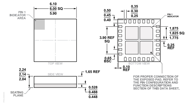
Figure 85. 28-Terminal Land Grid Array [LGA] (CC-28-4) Dimensions shown are in millimeters
