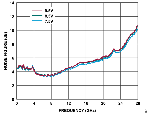
Figure 27. Noise Figure vs. Frequency Over V_{DD} , 200 MHz to 28 GHz, I_{DQ} = 90 mA, Mode = Internal Amplifier
