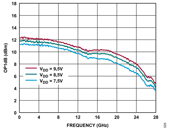
Figure 28. OP1dB vs. Frequency Over V_{DD} , 100 MHz to 28 GHz, I_{DQ} = 90 mA, Mode = Internal Amplifier
