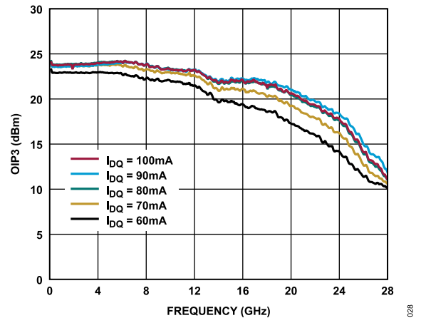
Figure 29. OIP3 vs. Frequency Over I_{DQ} , 100 MHz to 28 GHz, V_{DD} = 8.5 V, Mode = Internal Amplifier
