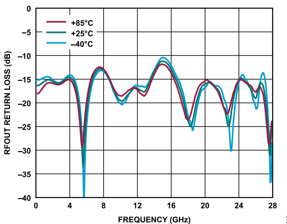
Figure 22. RFOUT Return Loss vs. Frequency Over Temperature, 200 MHz to 28 GHz, V_{DD} = 8.5\text{ V} , I_{DQ} = 90\text{ mA} , Mode = Internal Amplifier
