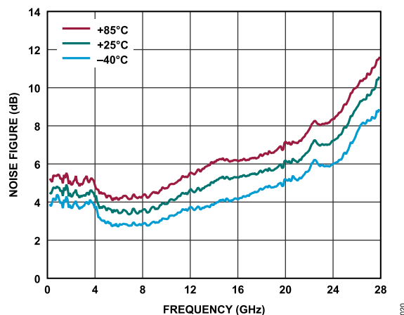
Figure 23. Noise Figure vs. Frequency Over Temperature, 200 MHz to 28 GHz, V_{DD} = 8.5\text{ V} , I_{DQ} = 90\text{ mA} , Mode = Internal Amplifier
