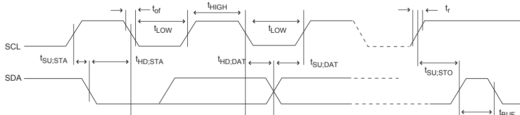
Figure 30-3. Two-wire Serial Bus Timing
