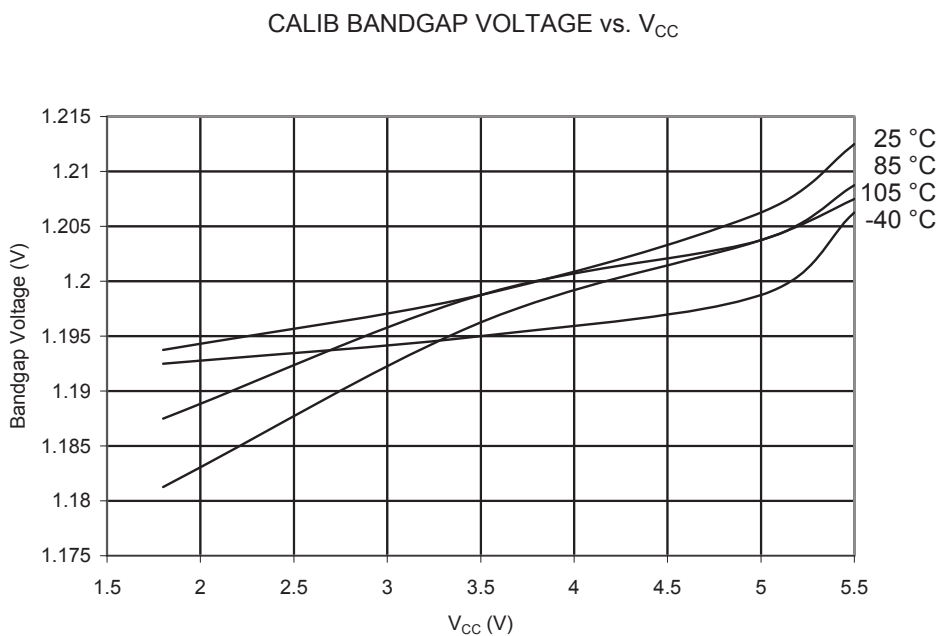
Figure 33-34. Bandgap Voltage vs. V CC
