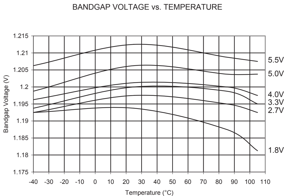
Figure 33-33. Bandgap Voltage vs. Temperature
