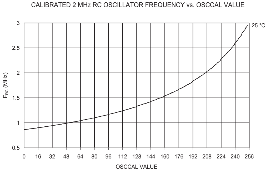
Figure 32-59. Calibrated 2MHz RC Oscillator Frequency vs. Oscscal Value
