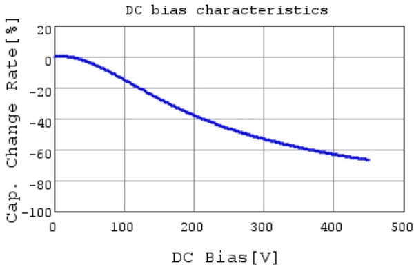
RDED72W473K2K1H03B C-DC bias capchange, 25.0
