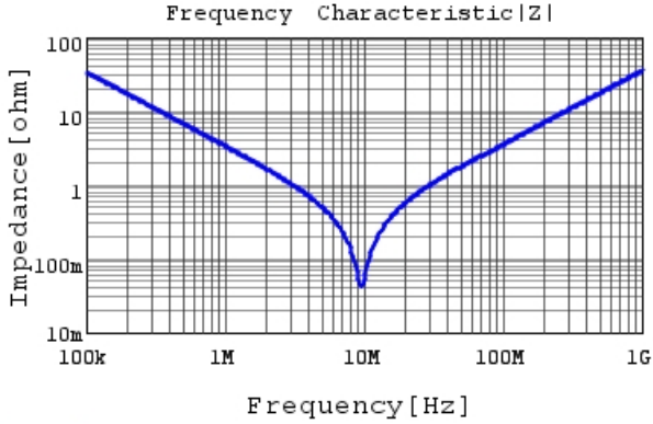
RDED72W473K2K1H03B |Z| DCOV, 25degC
