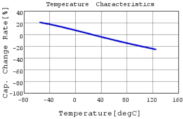
RDED72W473K2K1H03B C-Temp. capchange, DCOV,
