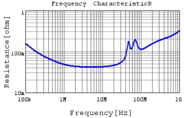
RDED72W473K2K1H03B R DCOV, 25degC
