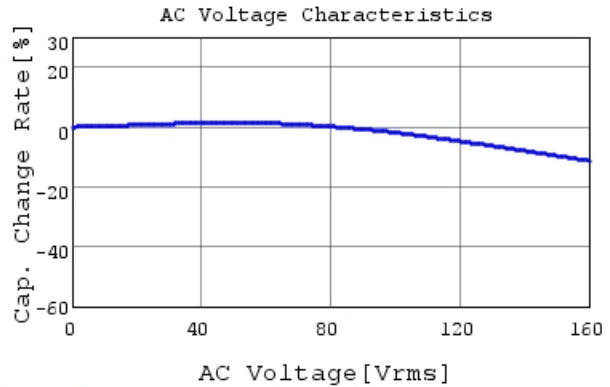
RDED72W473K2K1H03B C-AC Voltage capchange, I
