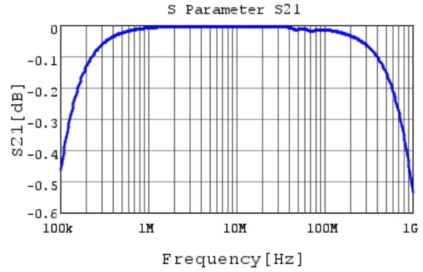
RDED72W473K2K1H03B S21 DCOV, 25degC
