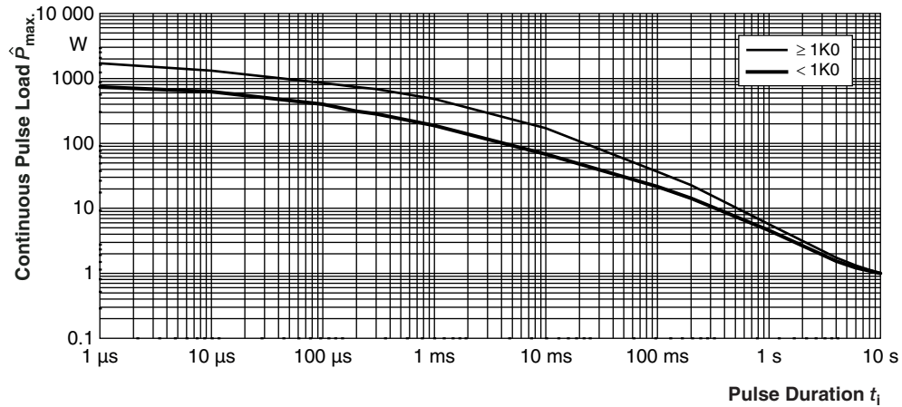
Maximum pulse load, continuous pulses; applicable if \bar{P} \leq P(\vartheta_{amb}) and \hat{U} \leq 4 kV; for permissible resistance change equivalent to 8000 h operation in power operation mode.
