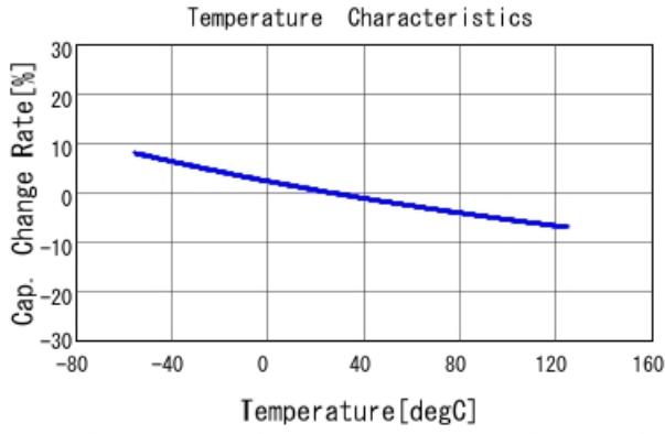
GCM31B7U2E103JX01 C-Temp. capchange, DC0V, AC1Vrms
