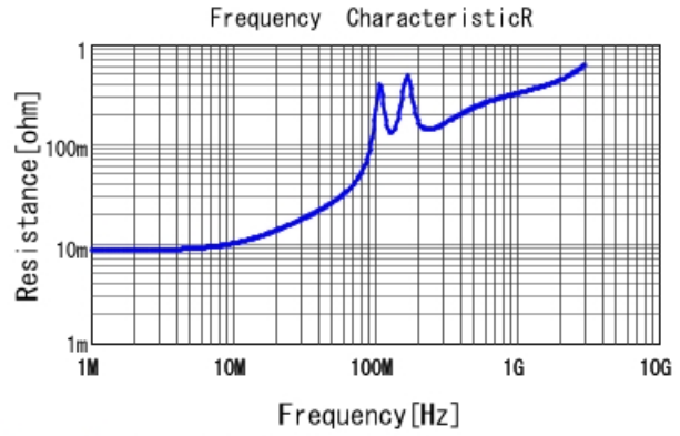
GCM31B7U2E103JX01 R DCOV, 25degC
