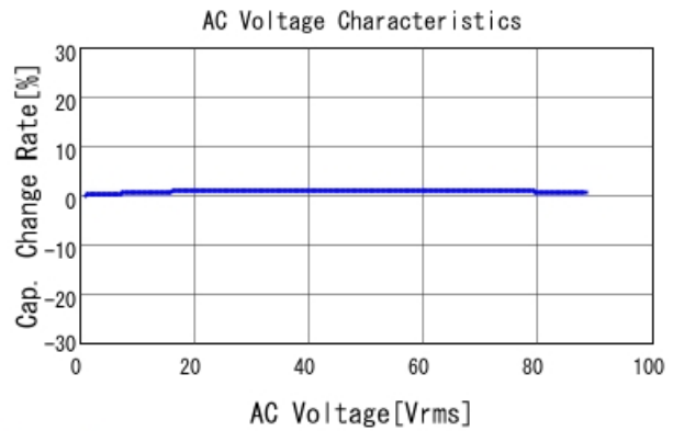
GCM31B7U2E103JX01 C-AC Voltage capchange, DCOV, 25
