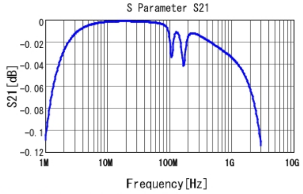
GCM31B7U2E103JX01 S21 DC0V, 25degC
