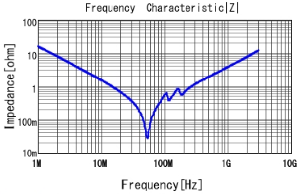
GCM31B7U2E103JX01 |Z| DCOV, 25degC
