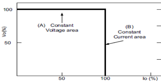
Typical LED power supply I-V curve
