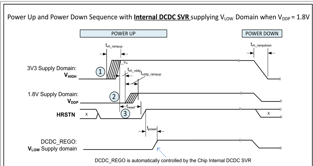
Figure 20 Timing Diagram for the Reset Sequence (Internal DCDC SVR Configuration) when V_{DDP}=1.8\text{ V}
