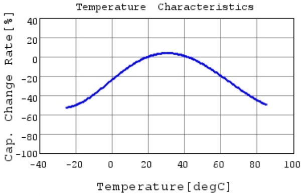
DE2E3KY102MN2AM01F C-Temp. capchange, DCOV,
