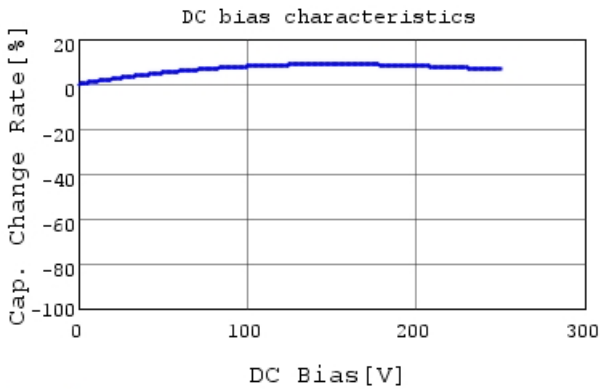
DE2E3KY102MN2AM01F C-DC bias capchange, 20.0
