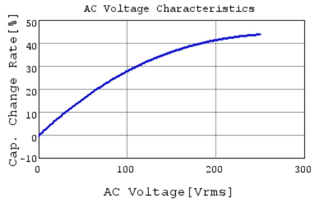
DE2E3KY102MN2AM01F C-AC Voltage capchange, I
