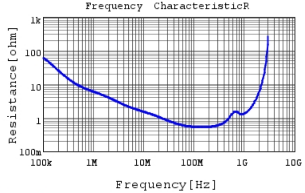
DE2E3KY102MN2AM01F R DCOV, 20degC
