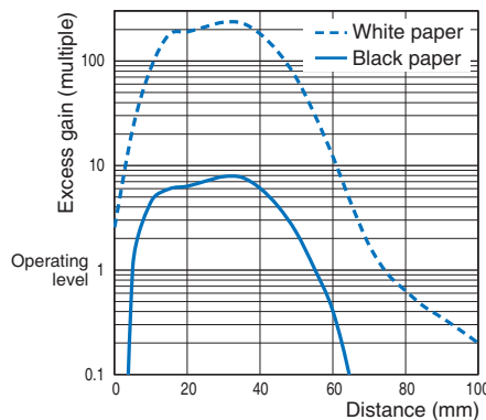
B5W-LB2112/LB2114/LB2122
