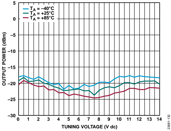
Figure 32. Output Power vs. Tuning Voltage at V_{CB} = 0\text{ V} for Various Temperatures
