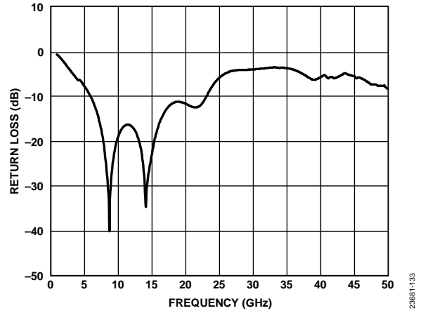
Figure 33. Return Loss vs. Frequency at V_{TUNE} = 6\text{ V}
