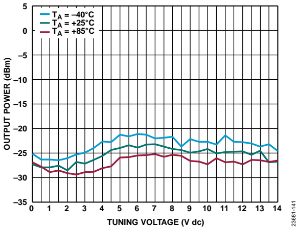
Figure 41. Output Power vs. Tuning Voltage at V_{CB} = 0\text{ V} for Various Temperatures
