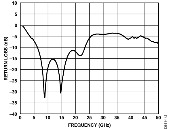
Figure 42. Return Loss vs. Frequency at V_{TUNE} = 6\text{ V}
