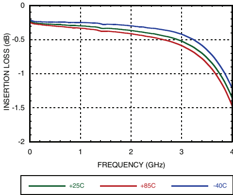
Insertion Loss
