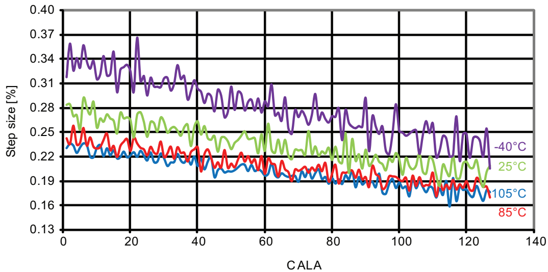
Figure 37-322. 2MHz internal oscillator CALA calibration step size.
