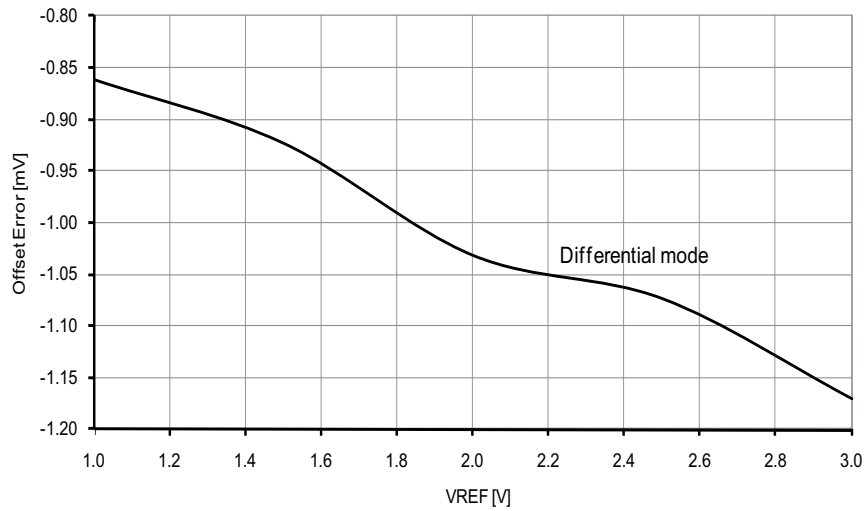
Figure 37-43. Offset error vs. V_{REF} . T = 25^\circ\text{C} , V_{CC} = 3.6\text{V} , ADC sampling speed = 500kps.
