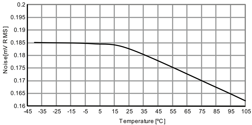
Figure 37-133. DAC noise vs. temperature.
