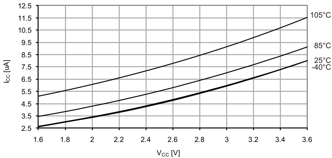
Figure 37-101. Standby supply current vs. V_{CC} .
