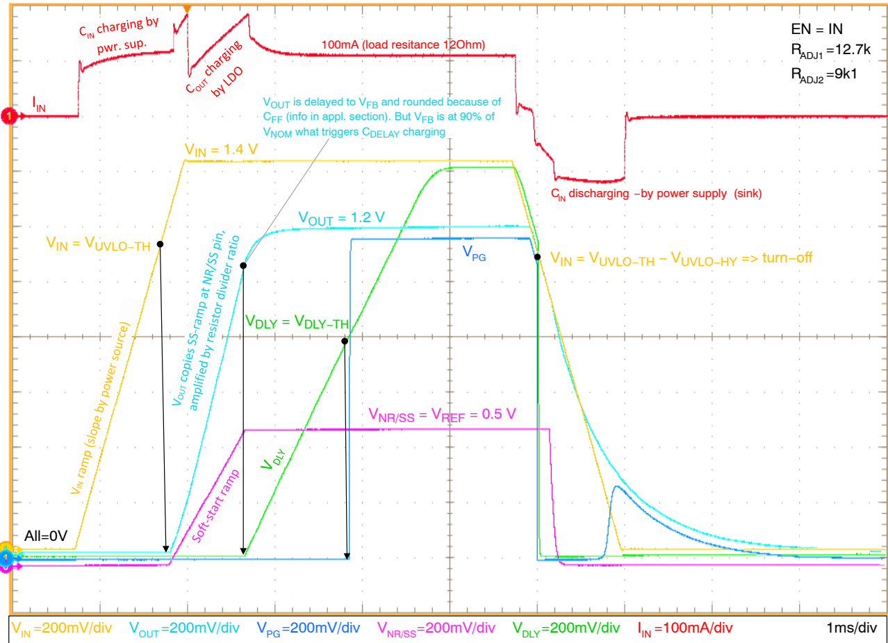
Figure 95. Start-up and Shut-down by V IN Voltage, ADJ Application, V NOM = 0.5 V, V OUT = 1.2 V
