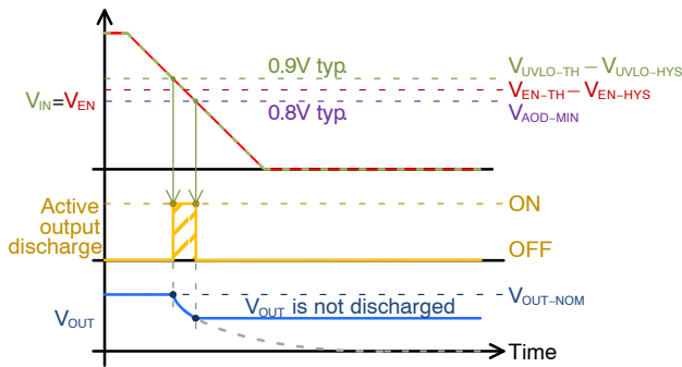
Figure 111. Active Output Discharge Activated by Falling V_{IN}
