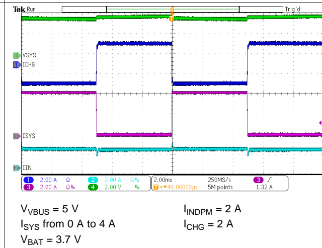
Figure 47. System Load Transient
