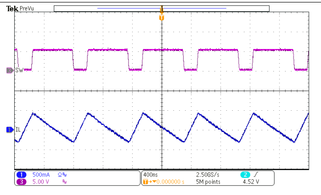
Figure 39. OTG Switching
