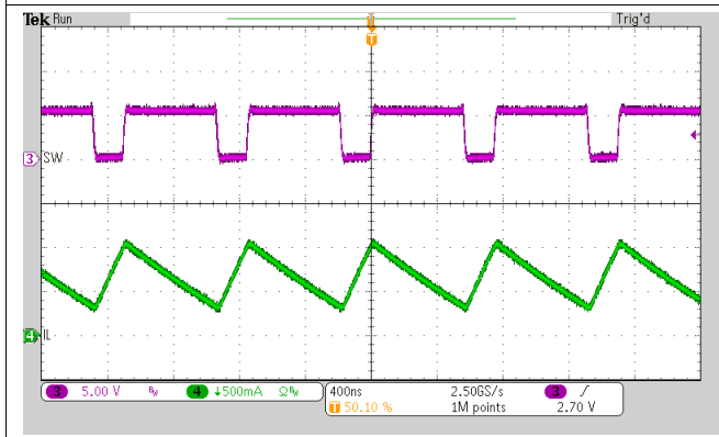
Figure 38. Charge Disable
