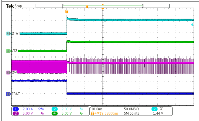
Figure 36. PWM Switching in Buck mode
