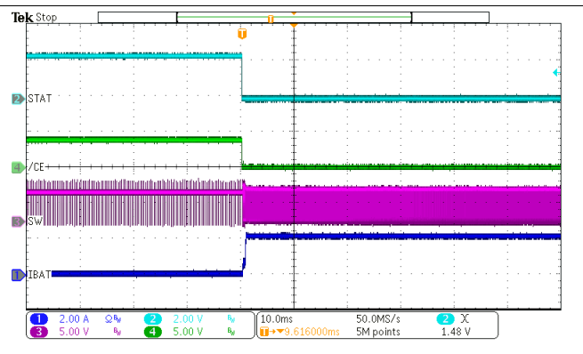
Figure 37. Charge Enable
