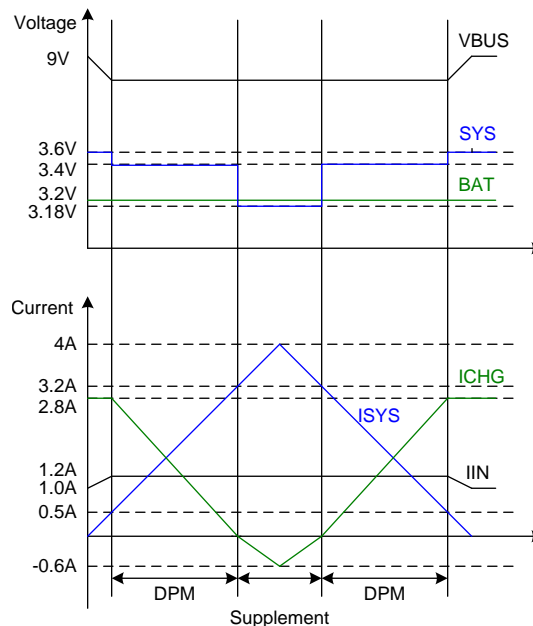
Figure 16. DPM Response
