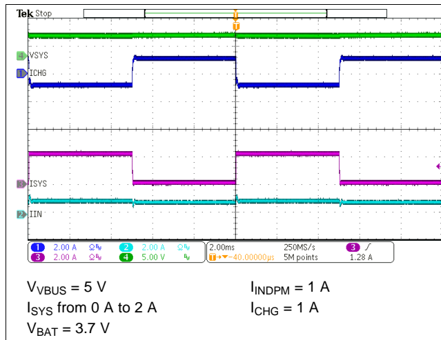
Figure 42. System Load Transient
