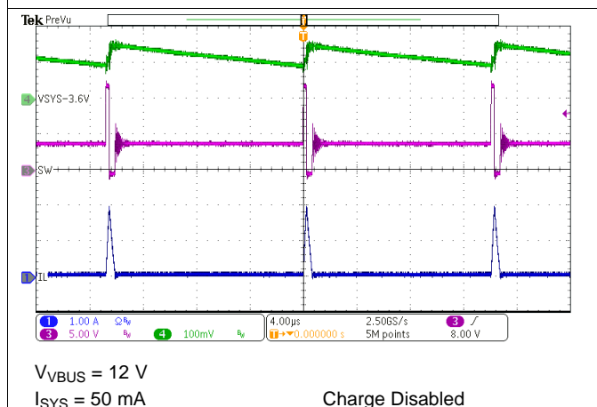
Figure 34. PFM Switching in Buck Mode
