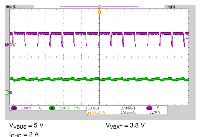
Figure 35. PWM Switching in Buck Mode
