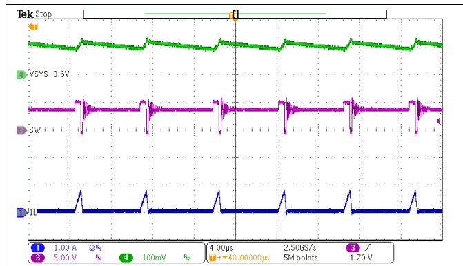
Figure 30. Power-Up with Charge Disabled
