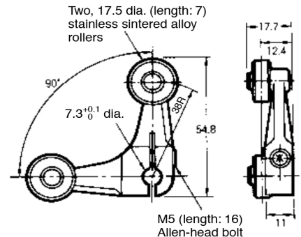
WL-5A104 has a resin roller
