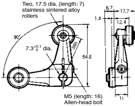
WL-5A100 has a resin roller
