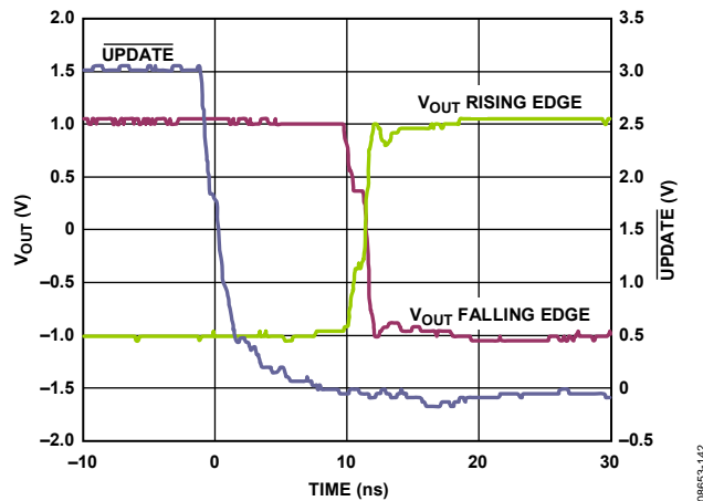
Figure 42. ADV3227 Switching Time
