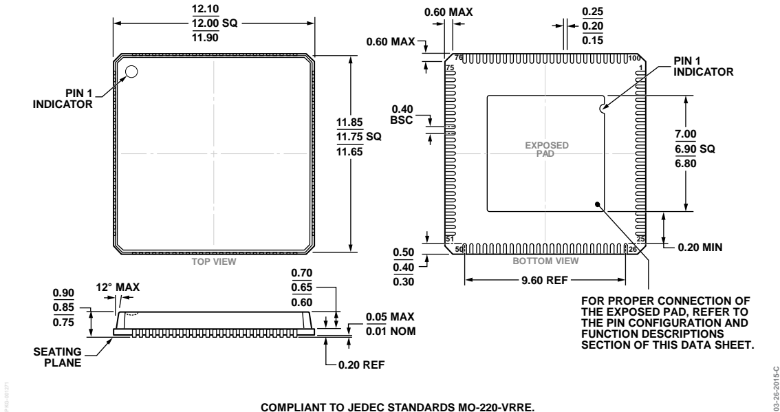
COMPLIANT TO JEDEC STANDARDS MO-220-VRRE. Figure 66. 100-Lead Lead Frame Chip Scale Package [LFCSP_VQ] 12 mm × 12 mm Body, Very Thin Quad (CP-100-1) Dimensions shown in millimeters
