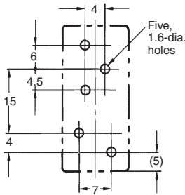
Mounting Holes (Bottom View)
