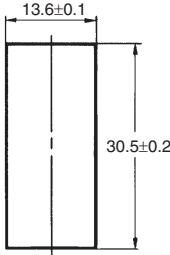
Panel Cutout (Bottom View)
