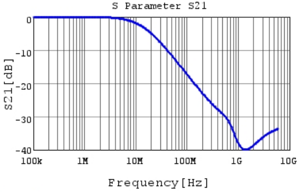
NFM21HC471R1H3 S21 DCOV,25degC, Feedthrough
