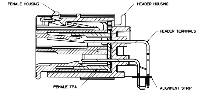
ASSEMBLY SECTION
