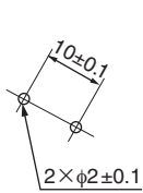
(PC board hole dimensions)
