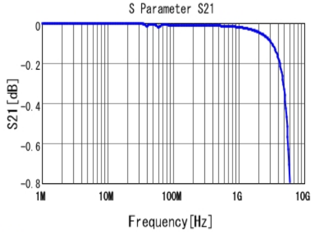
■ GRM31C5C1H683JA01 S21 DCOV, 25degC
