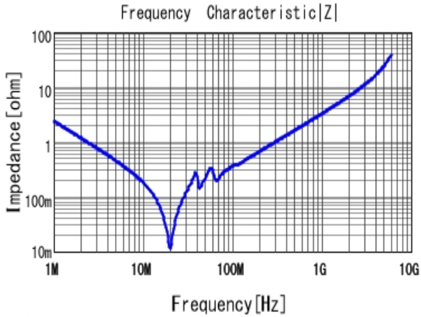
■ GRM31C5C1H683JA01 |Z| DCOV, 25degC
