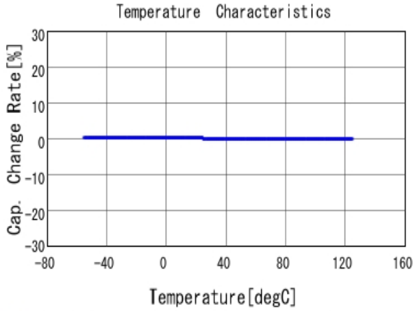
■ GRM31C5C1H683JA01 C-Temp. capchange, DCOV, AC1Vrms
