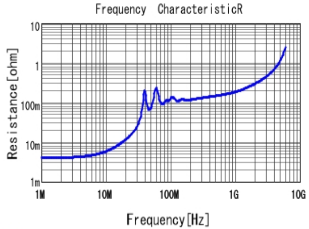
■ GRM31C5C1H683JA01 R DCOV, 25degC
