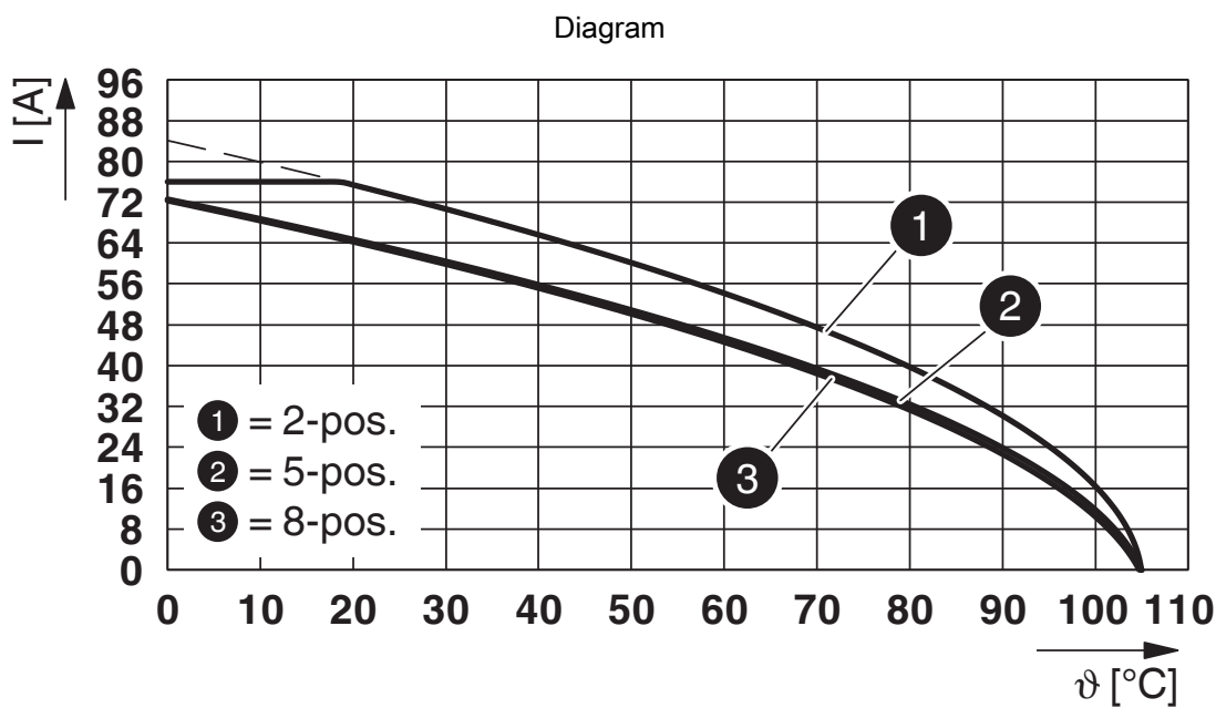
Type: PC 16/...-ST-10,16 with PC 6-16/...-G-10,16
