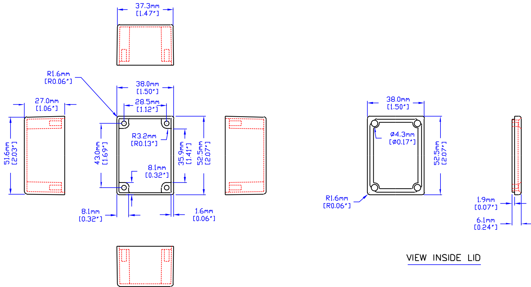
VIEW OF BOX (LID REMOVED)
