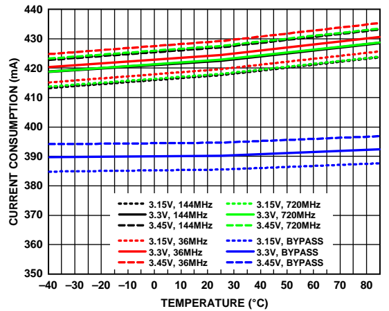
Figure 20. Current Consumption vs. Temperature for 36 MHz, 144 MHz, 720 MHz, and Bypass Mode
