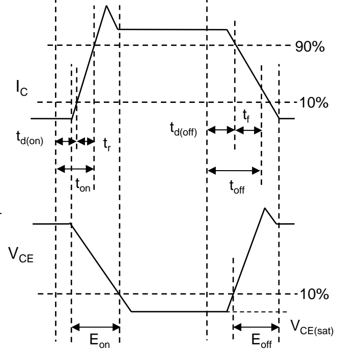
Fig.25 Inductive Load Waveform
