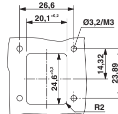
Dimensional drawing
