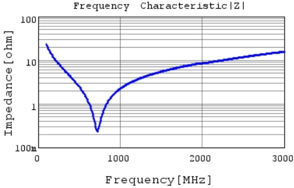
GRM21A5C2E680JW01 |Z| DCOV, 25degC
