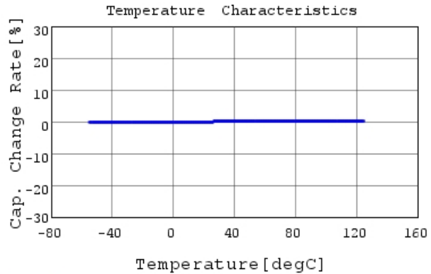
GRM21A5C2E680JW01 C-Temp. capchange, DCOV, 1
