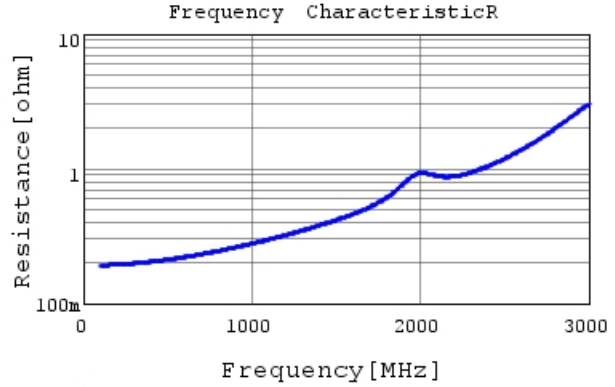
GRM21A5C2E680JW01 R DCOV, 25degC
