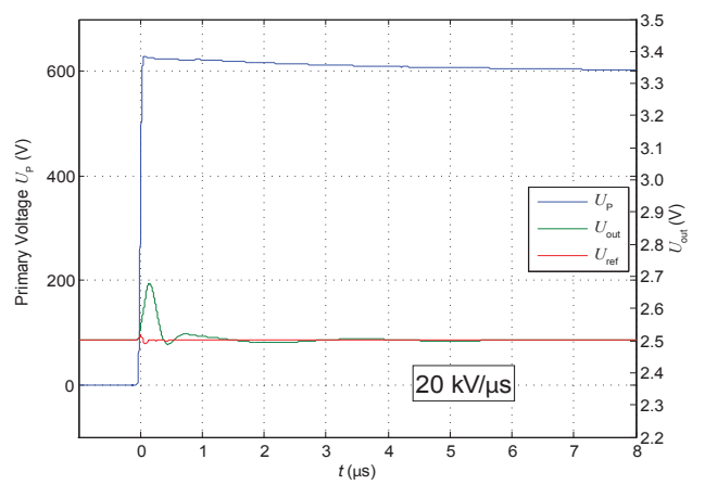
Figure 10: du/dt
