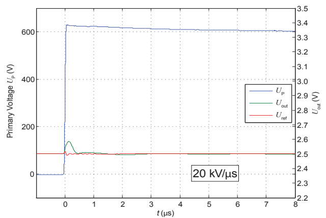
Figure 15: du/dt
