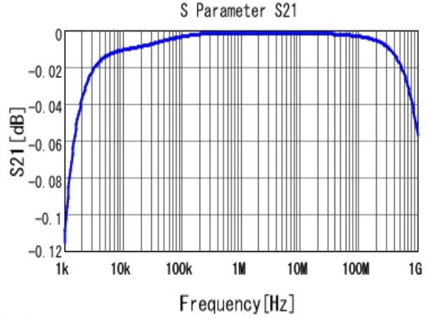
■ ECASD41A106M055K00 S21 DCOV, 25degC
