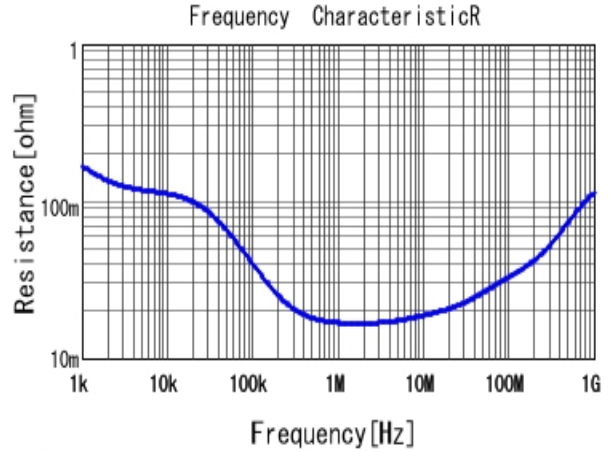
■ ECASD41A106M055K00 R DCOV, 25degC
