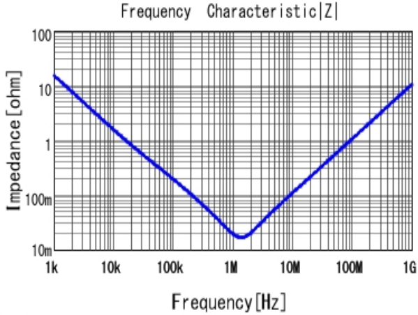
■ ECASD41A106M055K00 |Z| DCOV, 25degC
