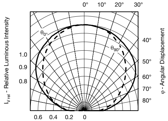
Fig. 20 - Relative Luminous Intensity vs. Angular Displacement
