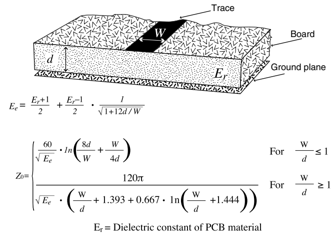
Figure 97: Microstrip Formulas
