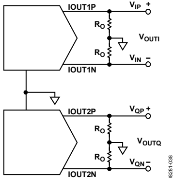
Figure 68. Basic Transmit DAC Output Circuit
