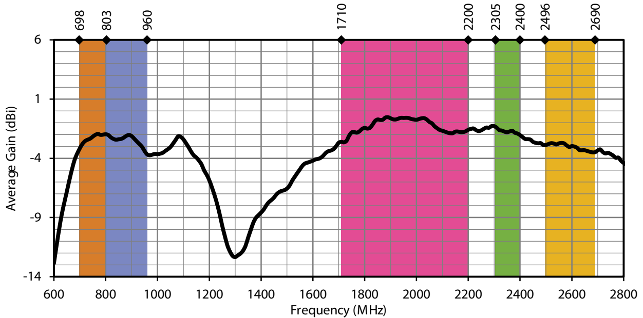
Figure 4. SP610 Average Gain with Frequency Band Highlights
