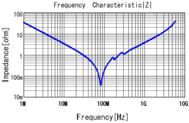
■ GRM3195C2A472JA01 |Z| DCOV, 25degC
