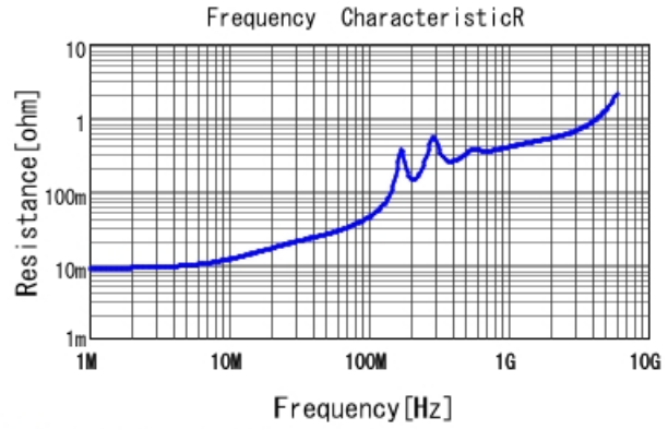
■ GRM3195C2A472JA01 R DCOV, 25degC
