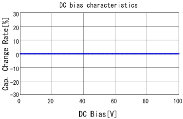
■ GRM3195C2A472JA01 C-DC bias capchange, 25.0degC, AC1V
