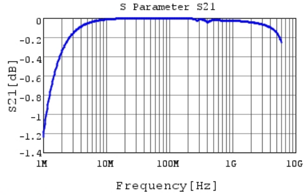
GRM1885C1H272JA01 S21 DCOV, 25degC
