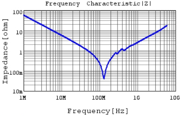
GRM1885C1H272JA01 |Z| DCOV, 25degC
