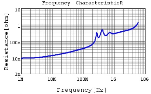
GRM1885C1H272JA01 R DCOV, 25degC
