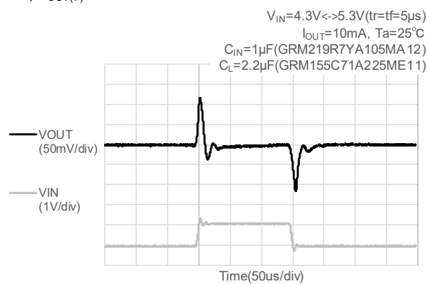
(11-2) V_{OUT(T)}=3.3V
