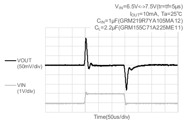
(11-3) V_{OUT(T)}=5.5V
