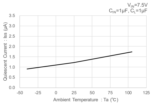
(2-3) V_{OUT(T)}=5.5V
