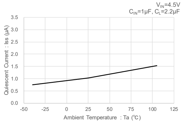
(2-1) V_{OUT(T)}=2.5V
