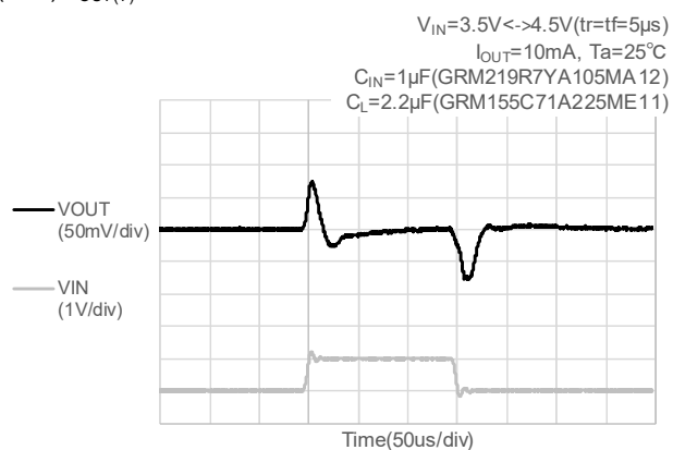
(11-1) V_{OUT(T)}=2.5V
