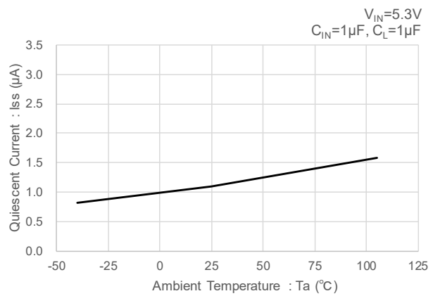
(2-2) V_{OUT(T)}=3.3V
