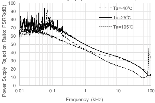
(14-3) V_{OUT(T)}=5.5V
