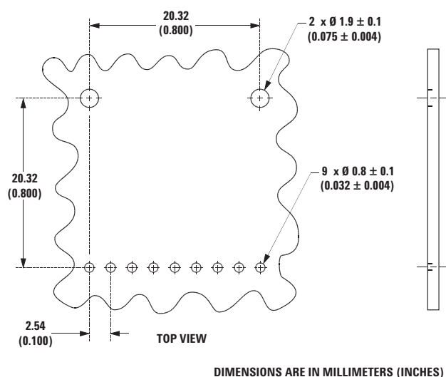
Figure 8a. Recommended Board Layout Hole Pattern
