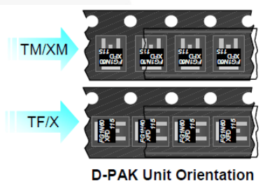
D-PAK Unit Orientation
