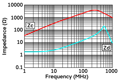
Impedance-frequency characteristics (DLW31SH222SQ2)
