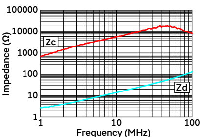
Impedance-frequency characteristics (DLW43SH101XK2)
