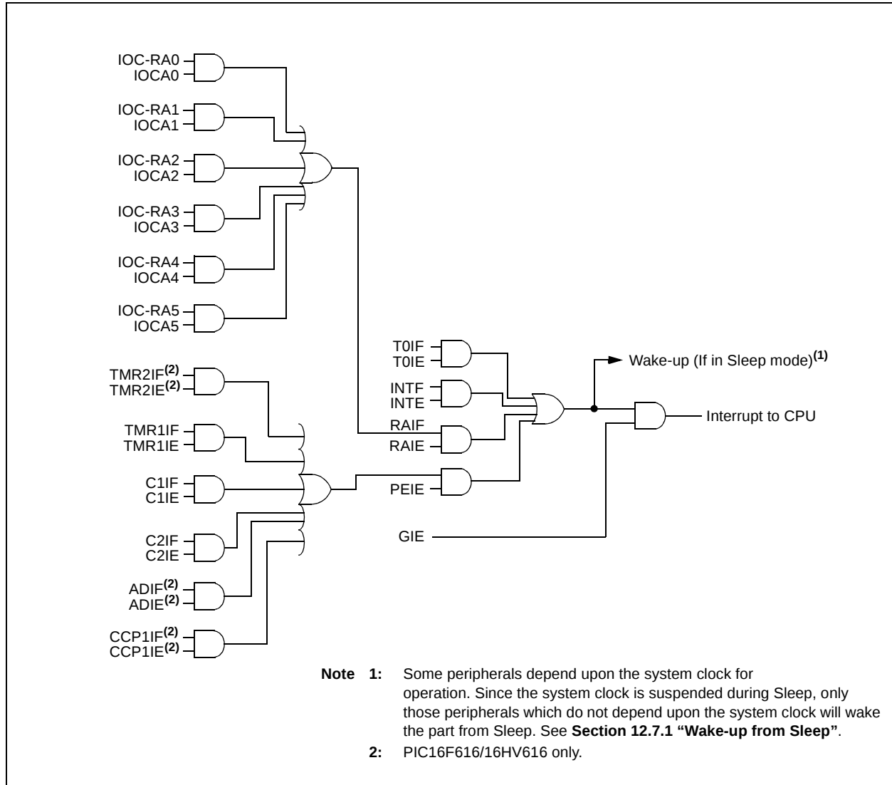
FIGURE 12-7: INTERRUPT LOGIC
