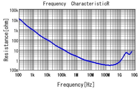
GCD188R71H102KA01 R DCOV, 25degC
