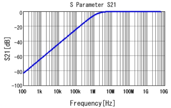
■ GCD188R71H102KA01 S21 DC0V, 25degC
