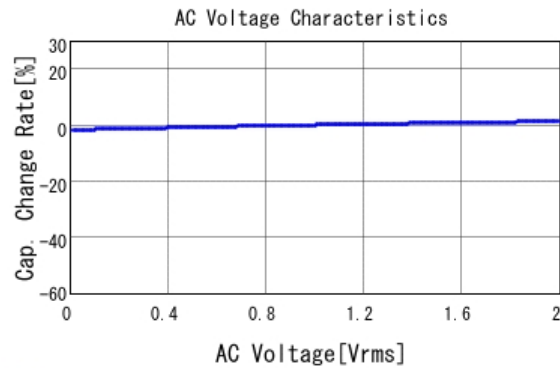
GCD188R71H102KA01 C-AC Voltage capchange, DCOV, 25.0d
