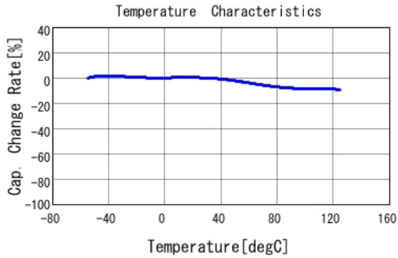
■ GCD188R71H102KA01 C-Temp. capchange, DC0.0V, AC1.0Vrm
