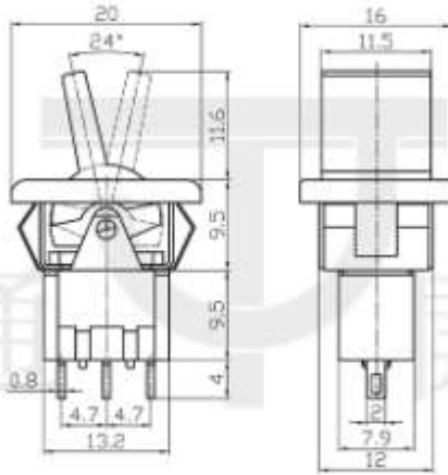
Outline Drawing
