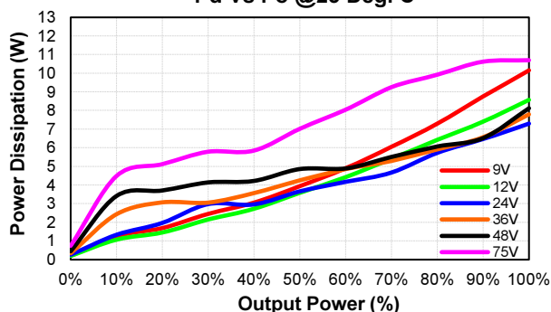
CQB75W8-36S48 Pd Vs P o @25 Deg. C
