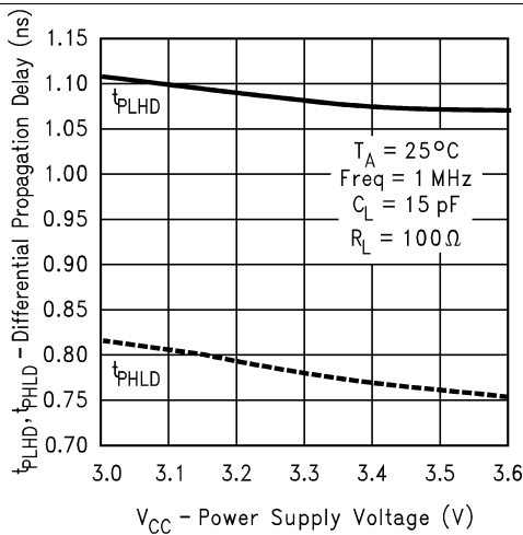
Figure 9. Differential Propagation Delay vs Power Supply Voltage
