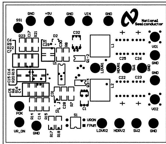
Figure 25. Top Overlay
