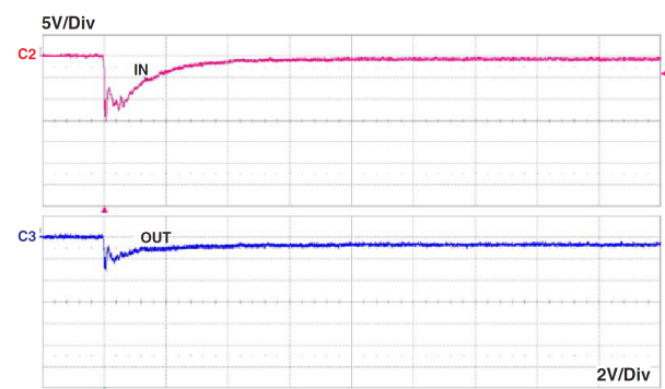
Figure 6. ESD response to IEC 61000-4-2 (-15 kV air discharge)
