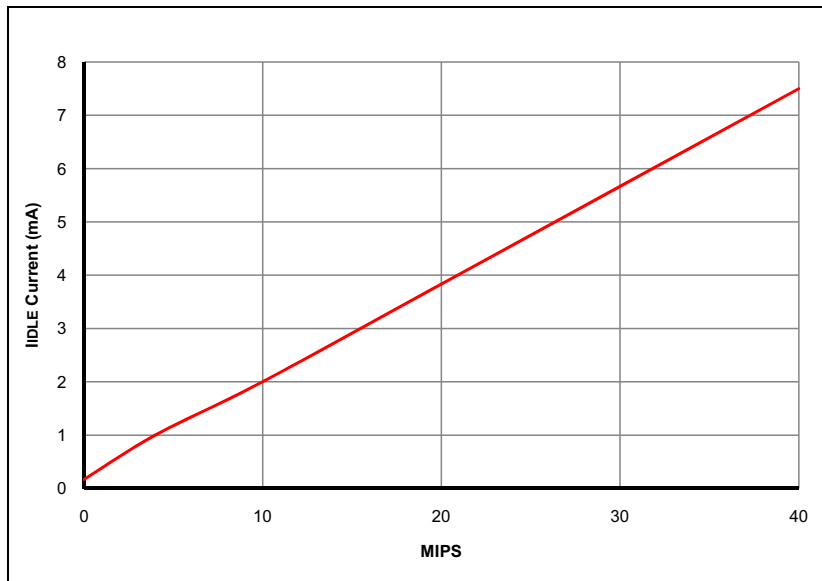
FIGURE 32-5: TYPICAL IDLE CURRENT @ VDD = 3.3V
