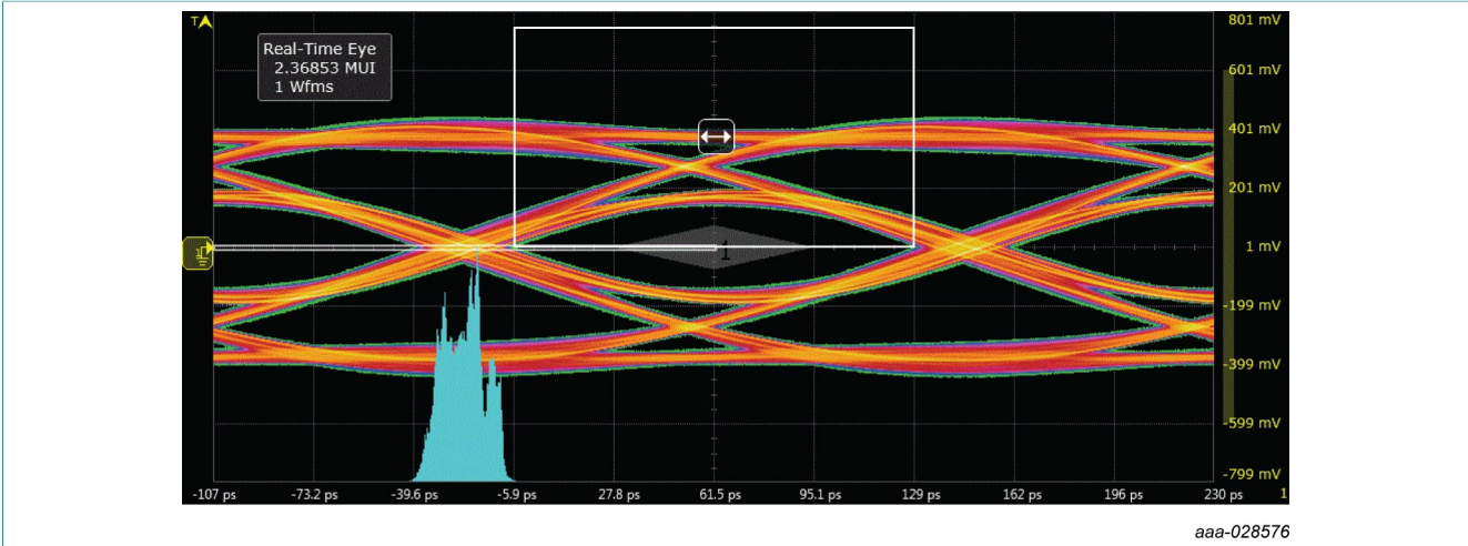
Fig. 11. HDMI 2.0 eye diagram TP2, test board without device; typical values
