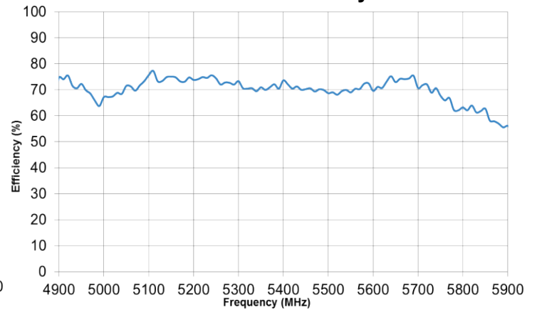
5 GHz Efficiency
