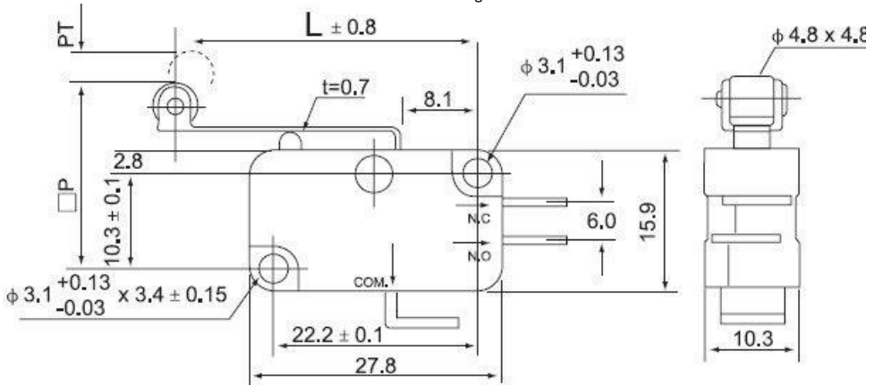
Outline Drawing
